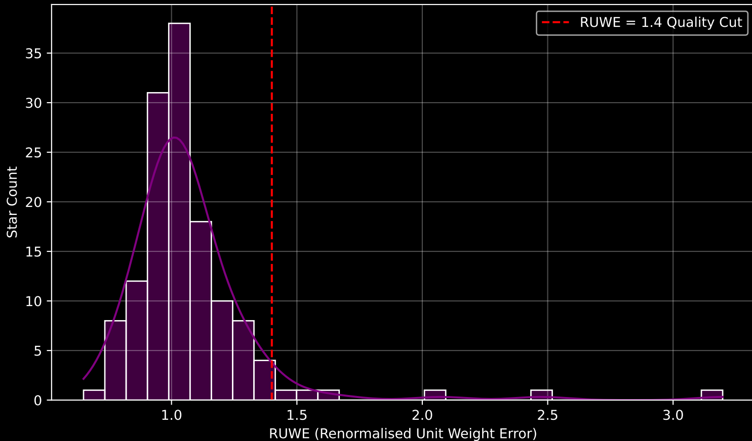
GAPOGEE DR17 Field [014-02] RUWE Distribution (n= 136)
