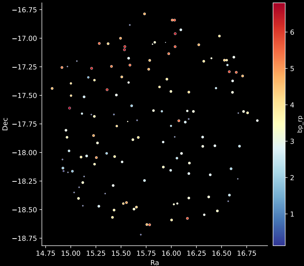
APOGEE DR17 Field: [014-02] Stars: 137
