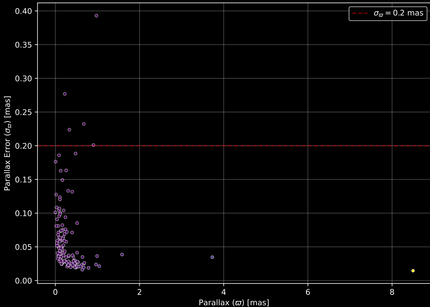
APOGEE DR17 Field: [014-02] Parallax Quality (n= 137)
