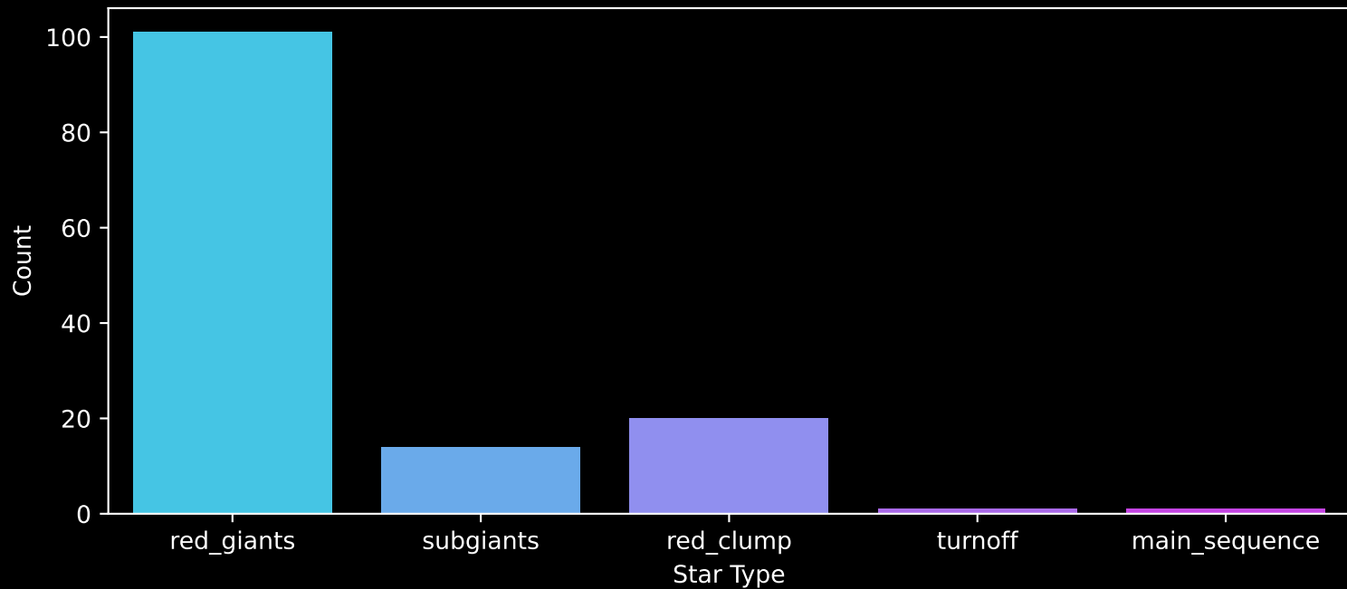
APOGEE DR17 Field: [014-02] Count plot of Star Type
