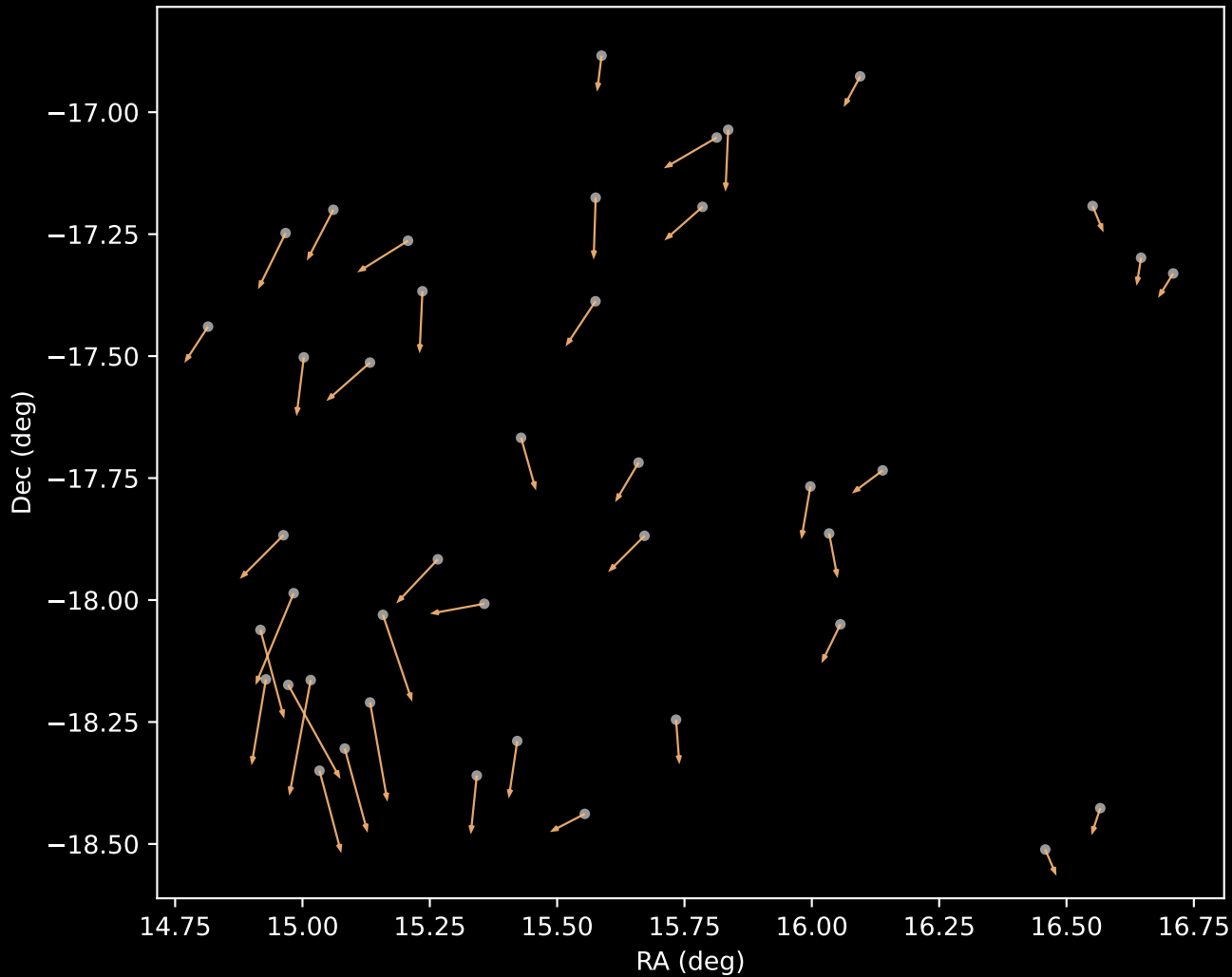
APOGEE DR17 Cluster 3 Proper Motion Vectors (n=42)
