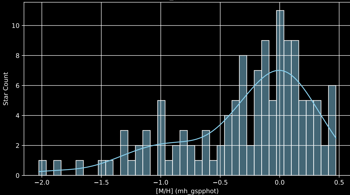
APOGEE DR17 Field: [014-02 [M/H] (mh_gspphot) (n= 126)
