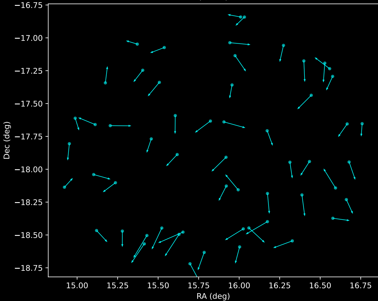
APOGEE DR17 Noise Stream Proper Motion Vectors (n=56)
