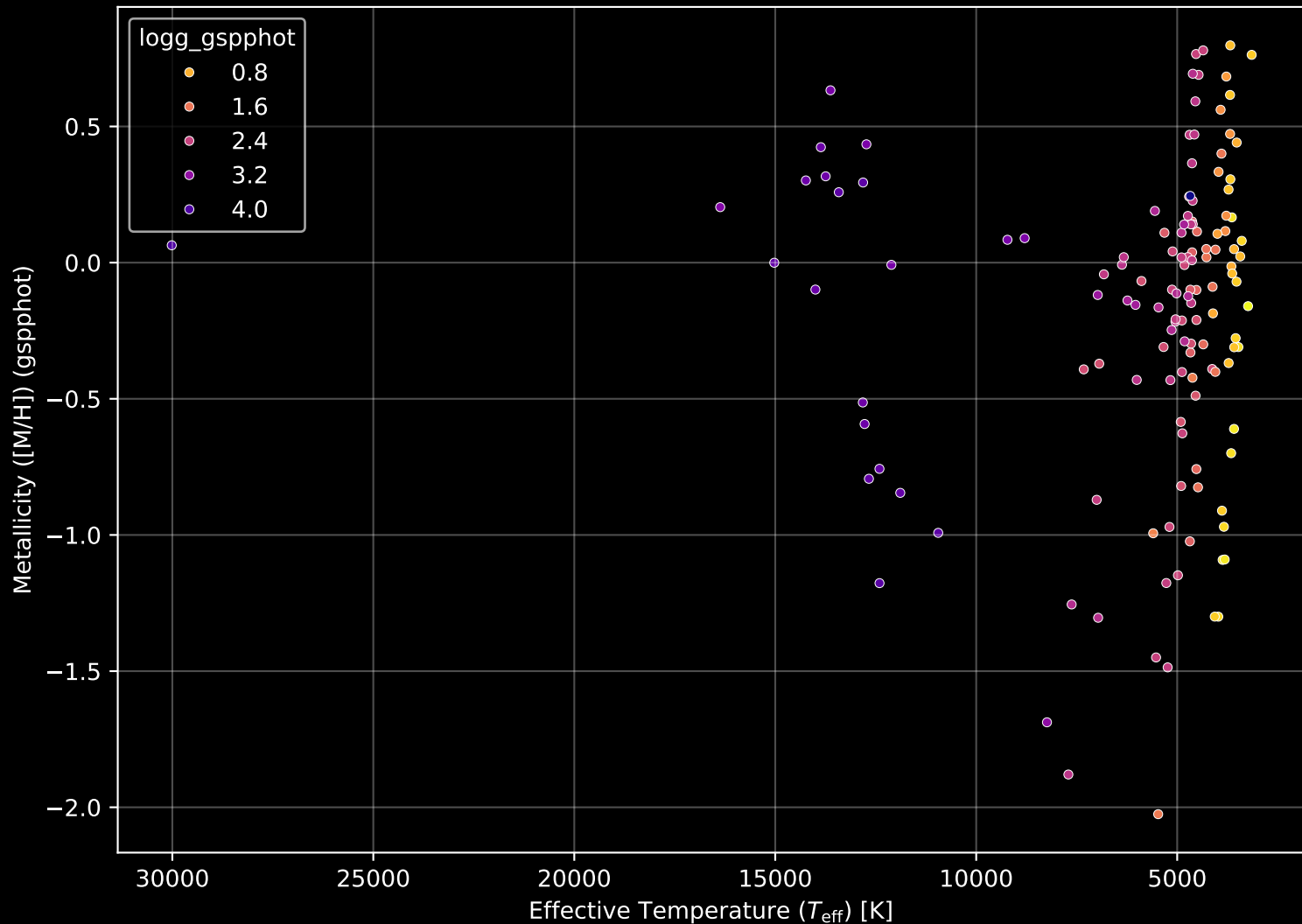
APOGEE DR17 Field: [014-02] Stellar Population Parameters (n= 137)
