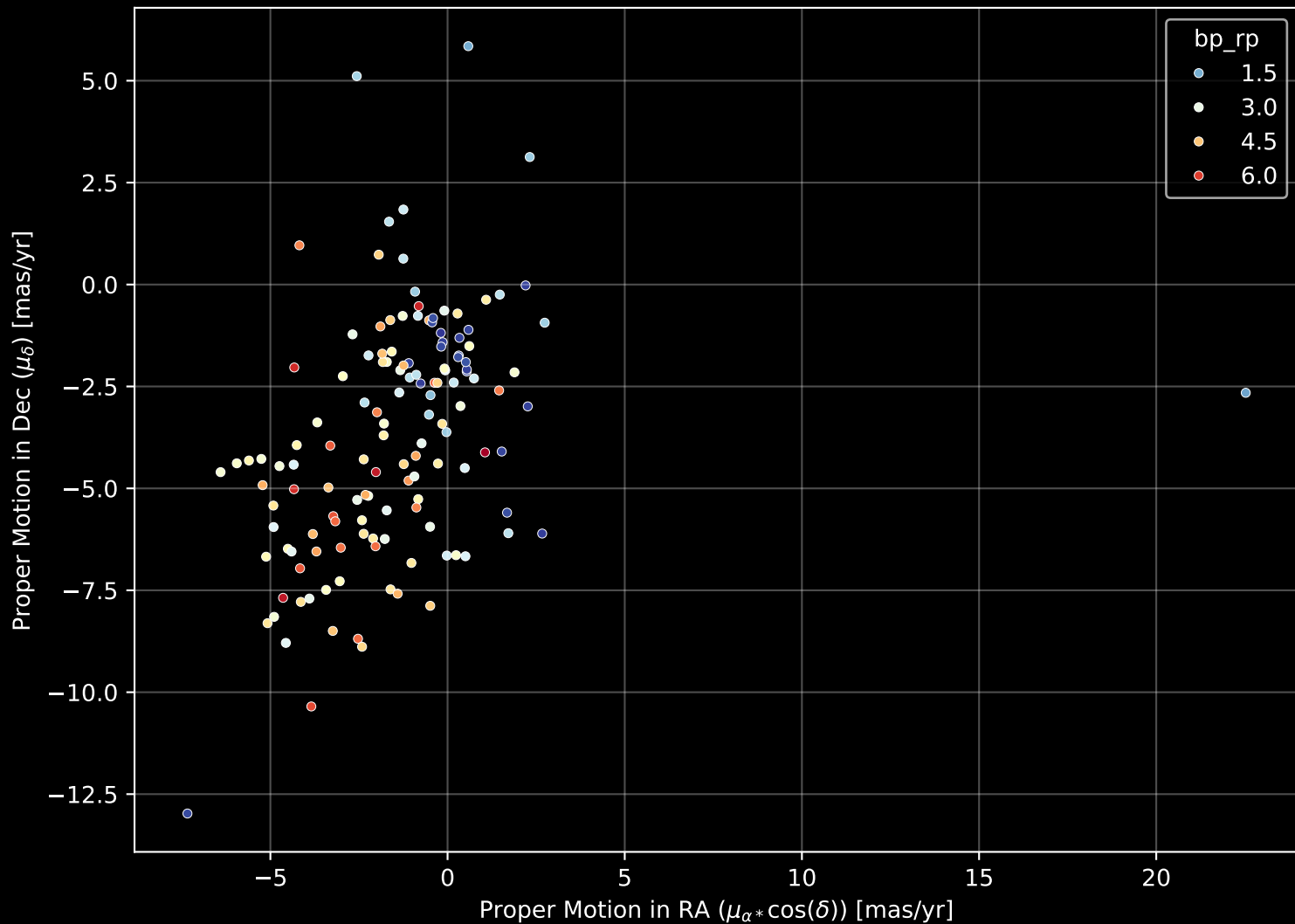
APOGEE DR17 Field: [014-02] Proper Motion Diagram (n= 137)
